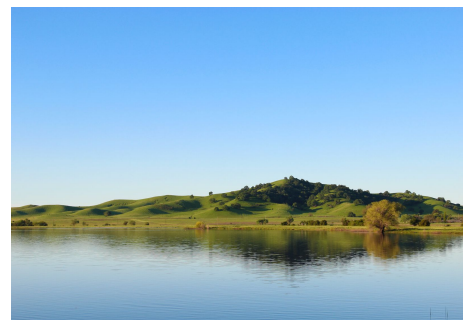
Clear sky
